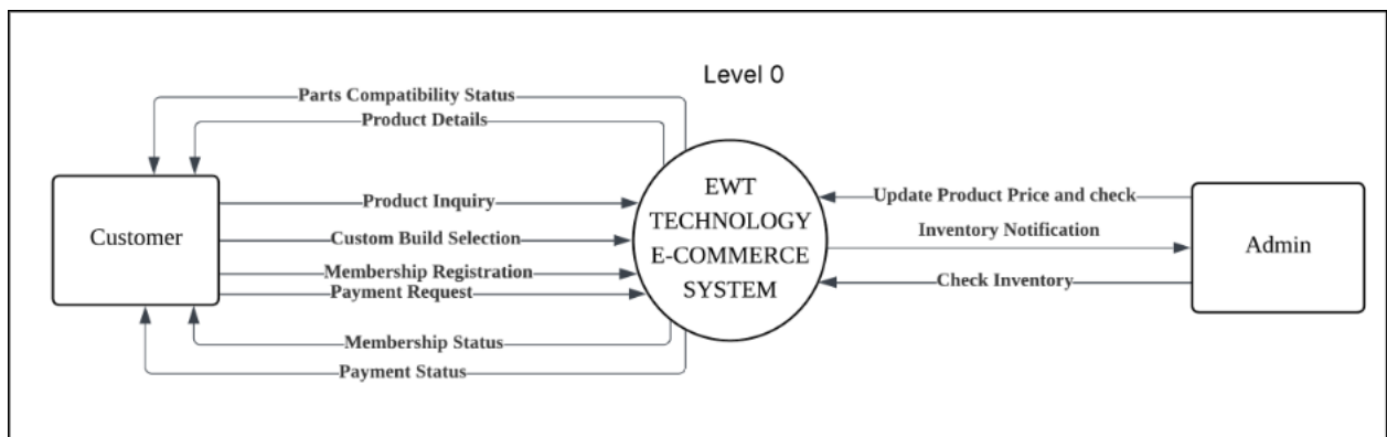
Figure 2.1.1 Context Diagram
